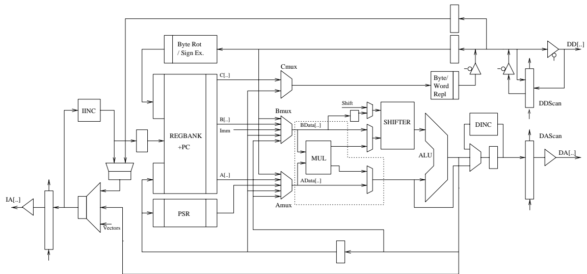
Figure 2 : The ARM9TDMI Datapath
