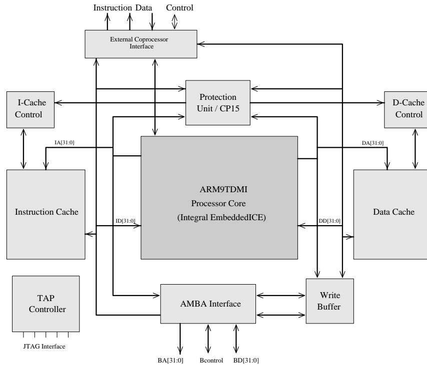
Figure 4 : The ARM940T Processor
