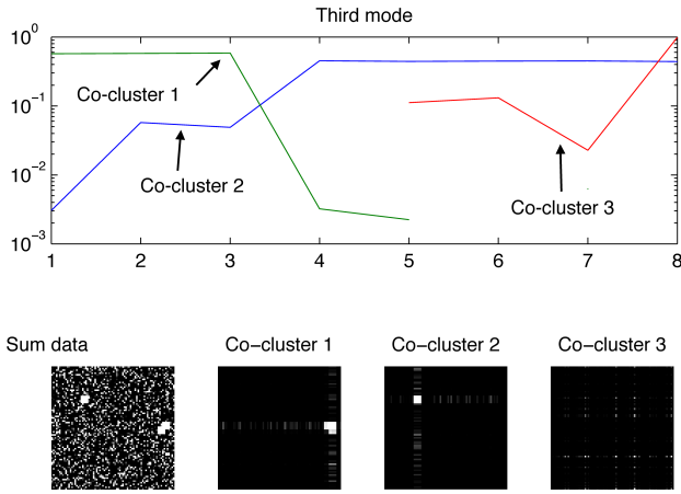
Fig. 5. Overlapping co-clusters: PARAFAC w/ NN ( \lambda = 0 ) [28], [37]
