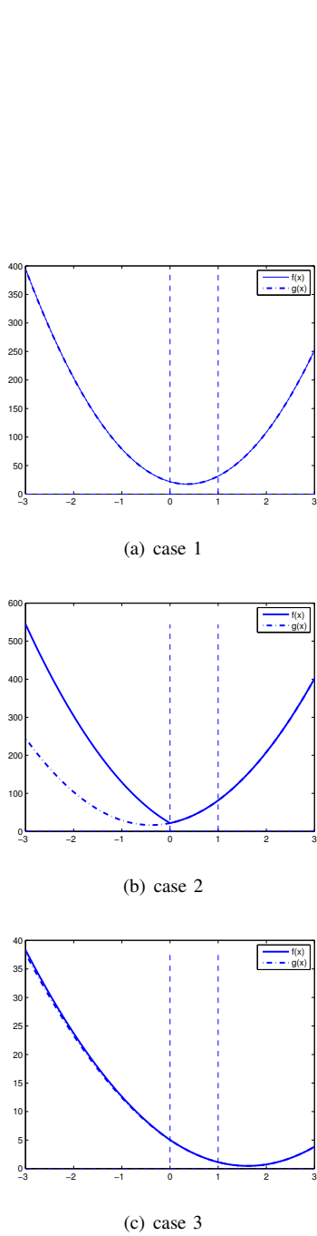
Fig. 2. Three cases for the [0, 1] constrained Lasso
