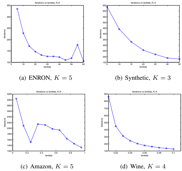
Fig. 8. Number of iterations vs \lambda , for fixed K
