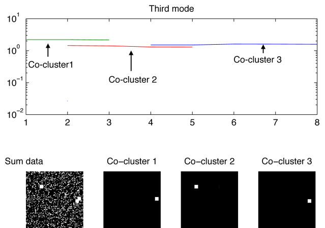
Fig. 4. Overlapping co-clusters: PARAFAC w/ NN SLF ( \lambda = 12 )
