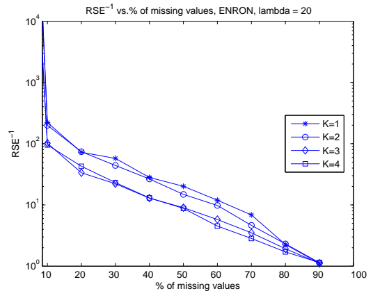
Fig. 10. RSE^{-1} (a signal-to-noise - like measure, see text) vs. % missing values
