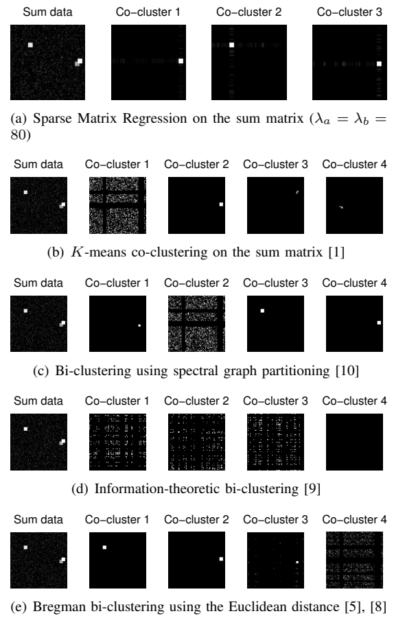
Fig. 3. Two-way co-clustering methods on synthetic data
