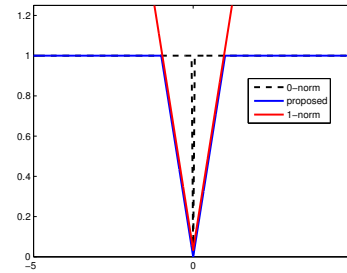
Fig. 1. Two approximations of the zero norm: note that the proposed one is much tighter for large |x| , due to saturation.
