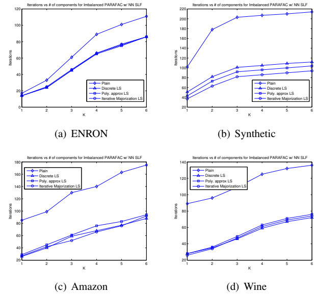
Fig. 9. Convergence speedup using line search, for fixed \lambda
