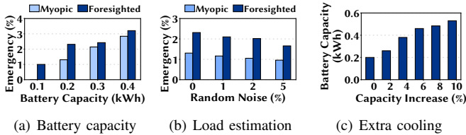
Fig. 12. Sensitivity of Foresighted. (a) Battery capacity. (b) Load estimation due to random noise in side channel. (c) Extra cooling capacity.
