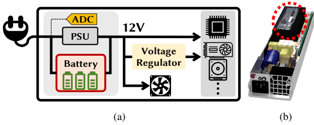
Fig. 4. (a) Attacker’s server with built-in batteries. (b) Supermicro’s power supply [17]. The built-in battery module is highlighted in a red circle.
