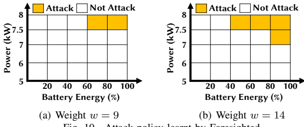
Fig. 10. Attack policy learnt by Foresighted.
