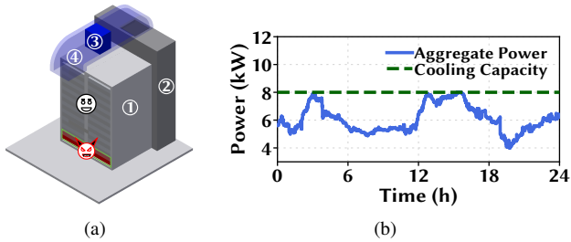
Fig. 6. (a) Data center layout. ① Server racks. ② Heat containment. ③ Air conditioner. ④ Supply air duct. (b) 24-hour snapshot of the power trace.
