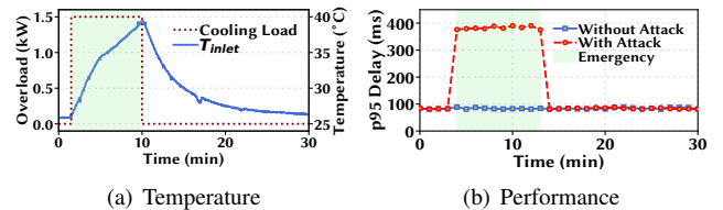
Fig. 13. Experiment in our server rack. (a) Server inlet temperature increases due to a cooling capacity overload by 1.5kW. (b) Latency performance is compromised due to server power capping for handling an emergency.
