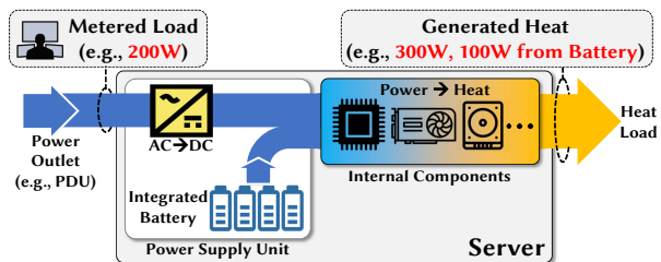
Fig. 1. An attacker uses its built-in batteries to stealthily inject additional heat to overload the cooling system.
