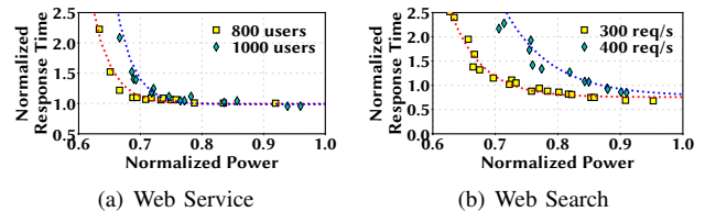
Fig. 14. Performance degradation due to power capping.
