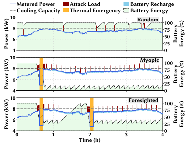
Fig. 9. 4-hour snapshot of thermal attacks.
