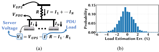
Fig. 5. (a) Server voltage carries the servers’ load information. (b) Load estimation error of the voltage side channel.
